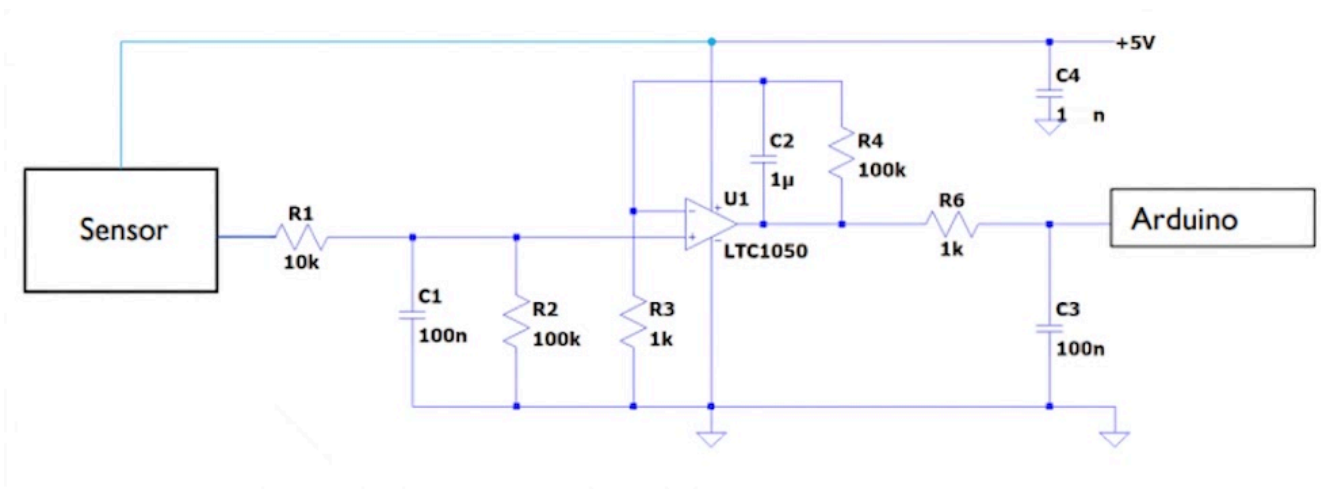
Figure 4: Proposed amplification circuit for measuring the signal
