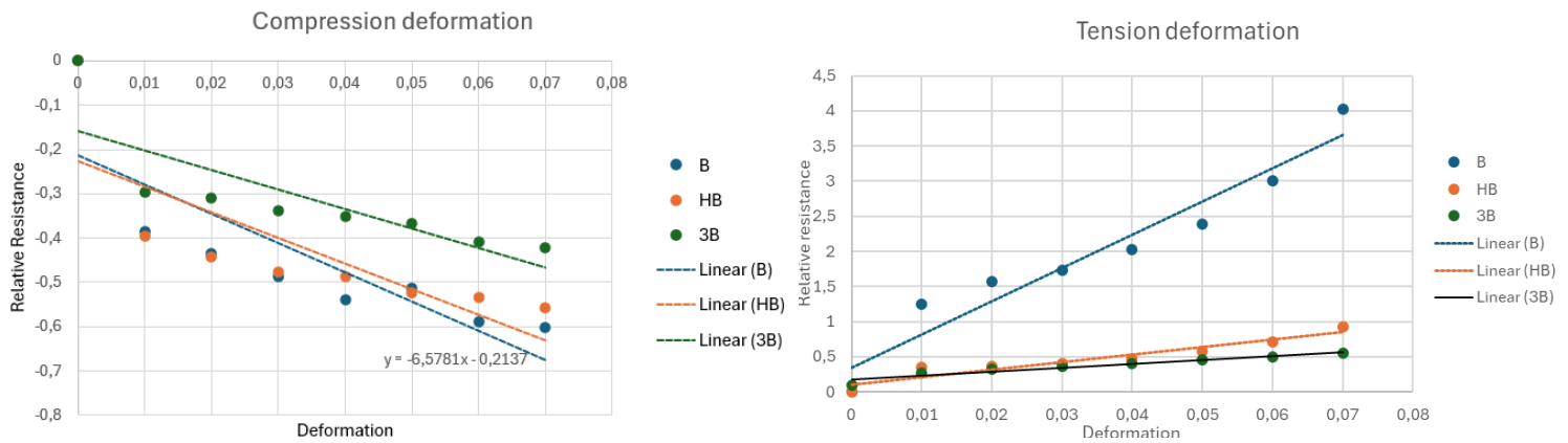
Figure 6,7: Characteristics graphs of resistance in standard test conditions
